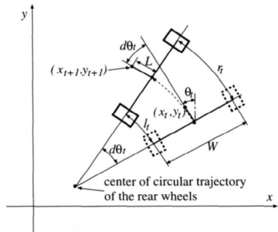
Fig. 8. Motion model of four wheeled mobile robot.
