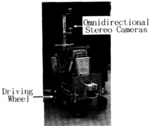
Fig. 7. Our mobile robot.
