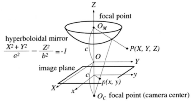
Fig. 2. Geometry of hyperboloidal projection. 11)
