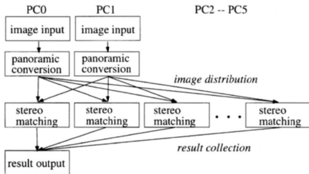
Fig. 5. PC cluster implementation.
