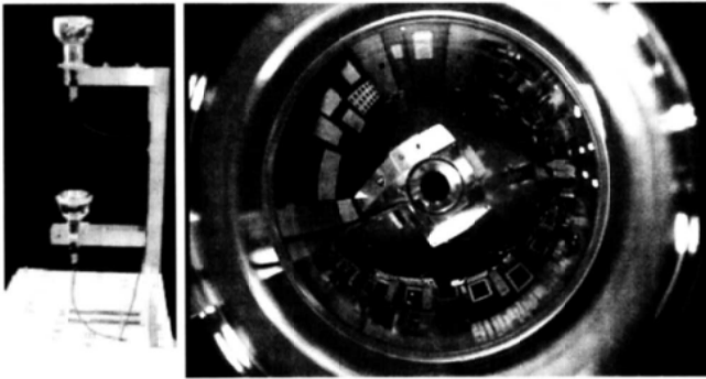
Fig. 1. Omnidirectional stereo setup and an example input image.
