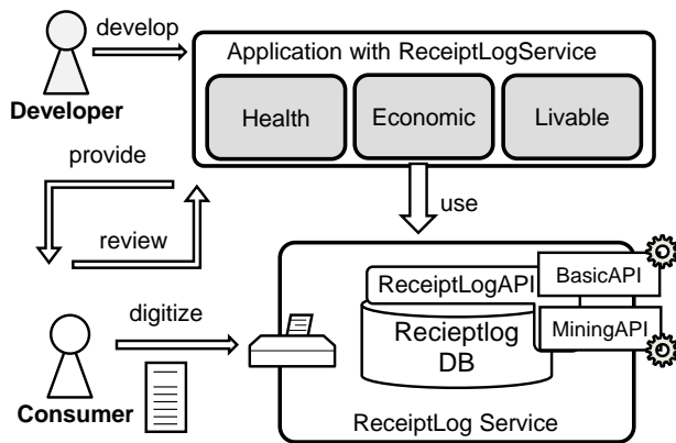
Fig. 1. Architecture of ReceiptLogService.
