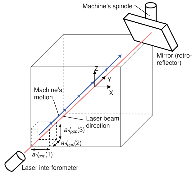
Fig. 4. Diagonal test [44].
