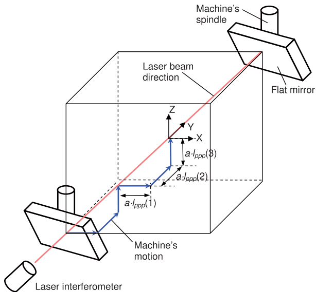
Fig. 5. Step-diagonal test [44].
